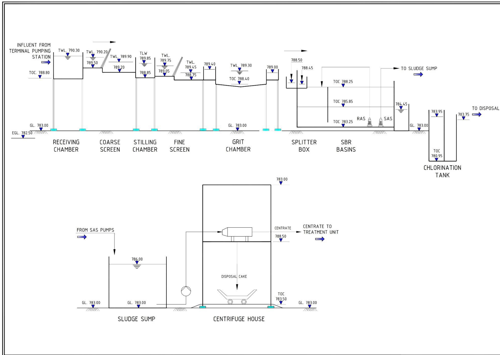
Fig. II (b): Sample Hydraulic Flow Diagram of STP
