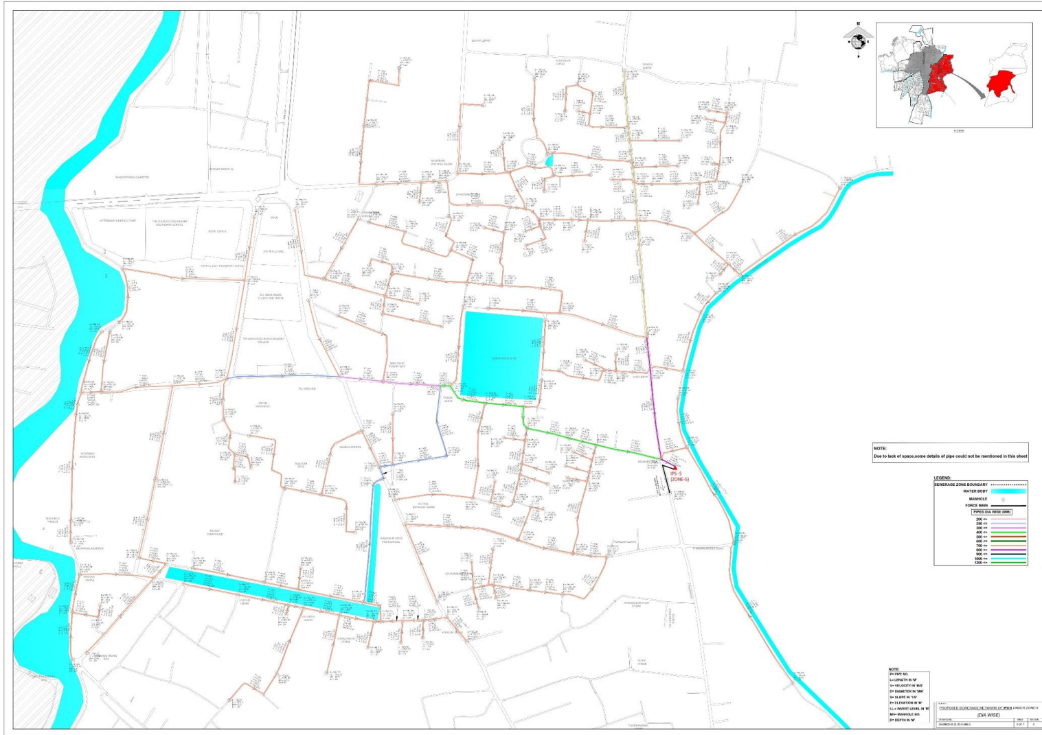
Fig. II(a): Sample drawing for sewer network
